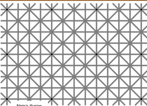
Ninio's illusion
