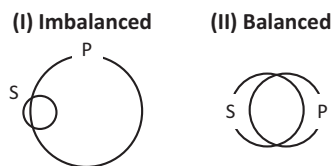
Fig. 1. Probabilistic structures.
