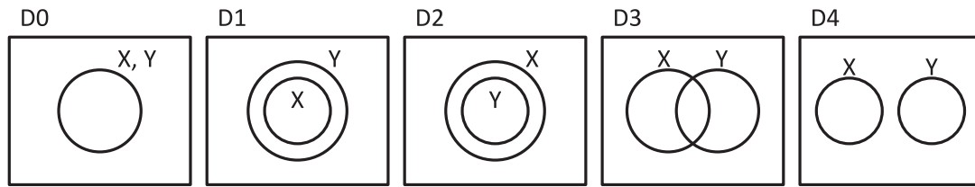
Fig. 3. Euler circles representing the relationships between two sets, X and Y.
