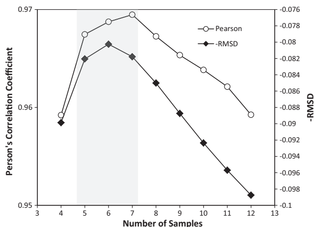
Fig. 14. The goodness-of-fit of the probabilistic representation model to data as a function of working memory capacity. Working memory capacity is assumed to be the number of samples in the SMM. Data for model fitting were taken from eight experiments in the literature, as introduced in Meta-Analysis 2.
