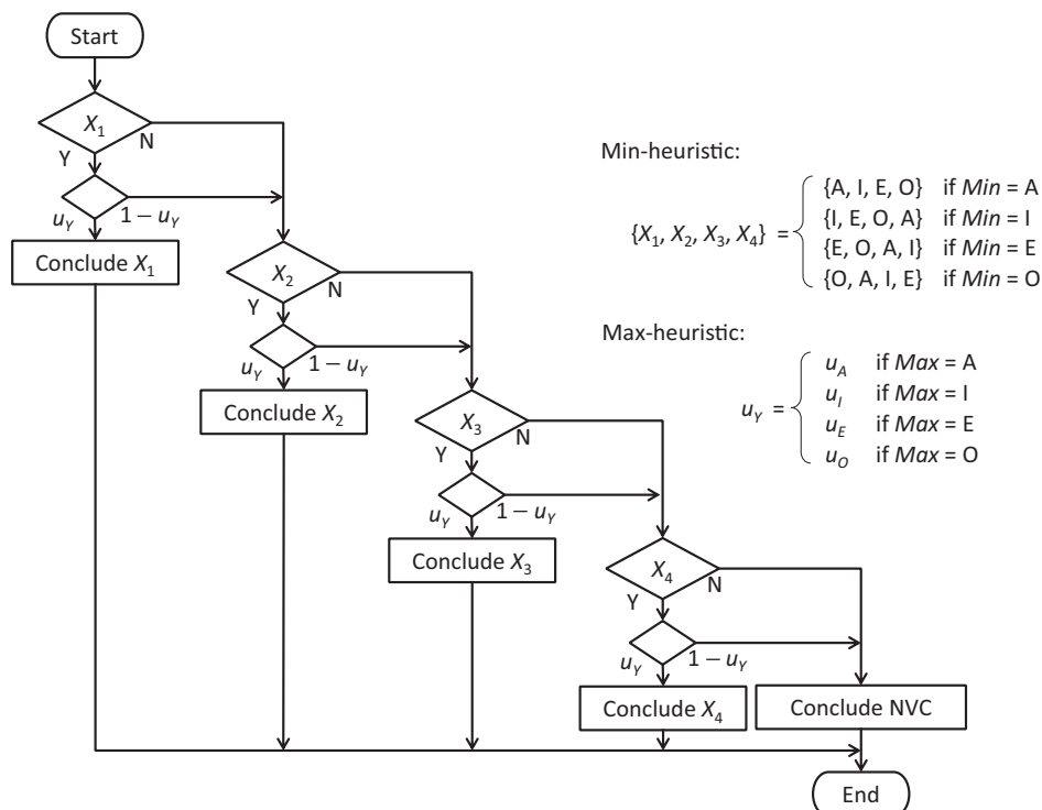
Fig. 8. The process for generating a logical conclusion in the model. Logical conclusions are determined by the order of the tests, the result of each test (depending on the contents of the SMM), and a random effect prescribed by free parameters ( u_A , u_I , u_E , and u_O ).
